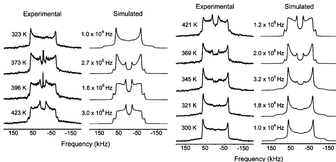
Figure 3. Experimental and simulated quadrupolar spin-echo solid-state ^2\text{H} NMR spectra of 1a during heating and transformation into 1b (left) and of 1b during cooling (right).
